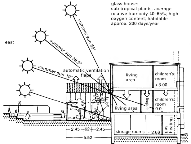
5 Solar town house with winter gardens for two storeys
